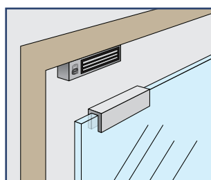
U Bracket
