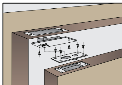
Embedded Installation
