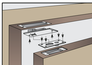
Embedded Installation
